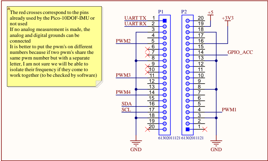
Raspberry pico Connector
