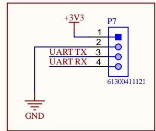
Pin Header UART
