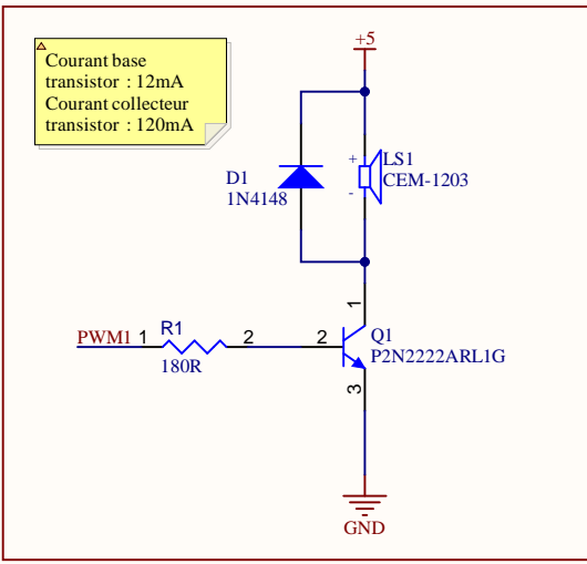
Buzzer
