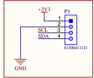
Pin Header I2C
