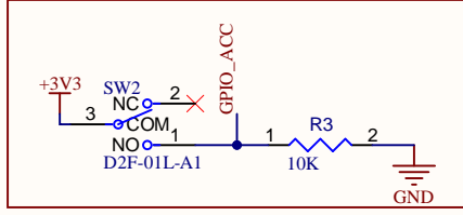
Accelerator contact
