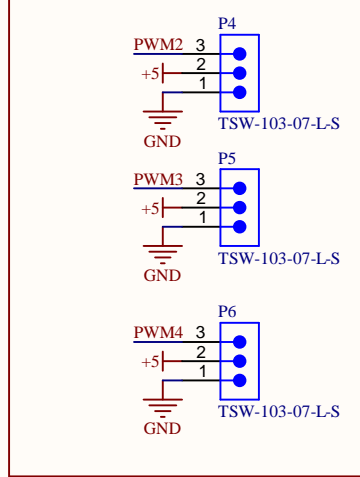
Pin Header Servo Motor
